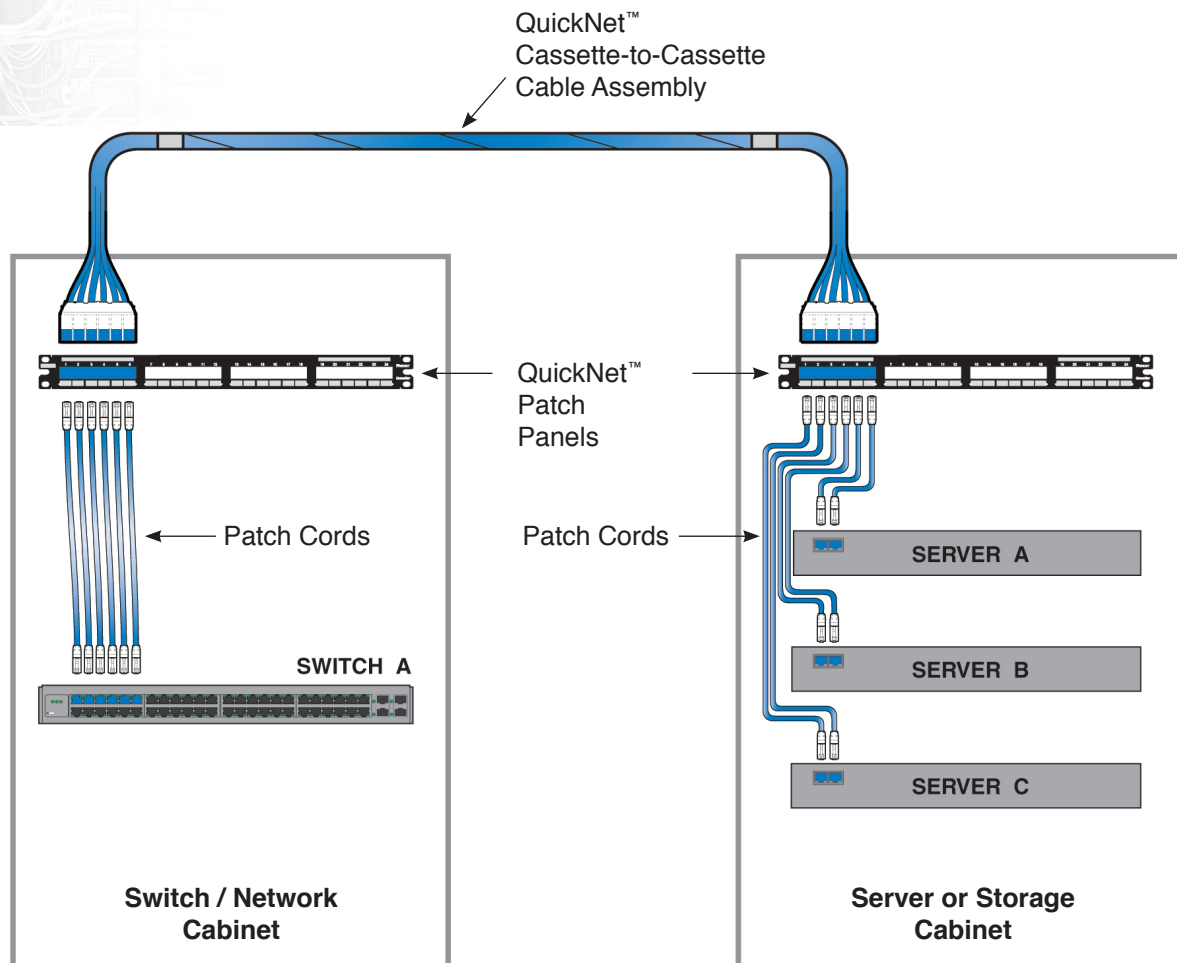
Figure 1 - Two-Connector Interconnect
