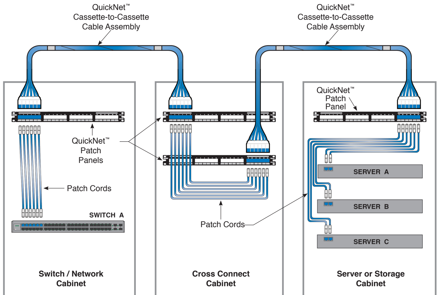
Figure 3 - Four-Connector Cross Connect
