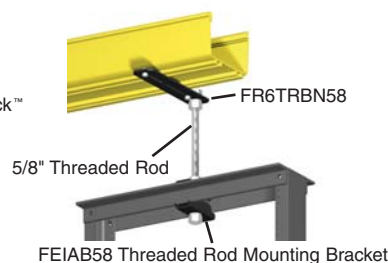
Mounting to EIA Racks
