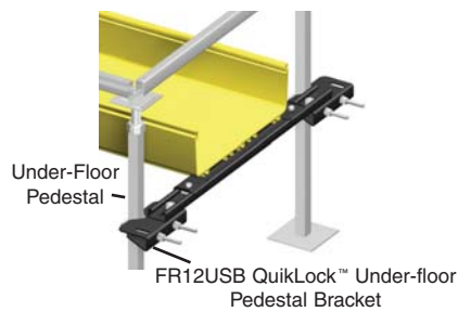
Under-Floor Support
