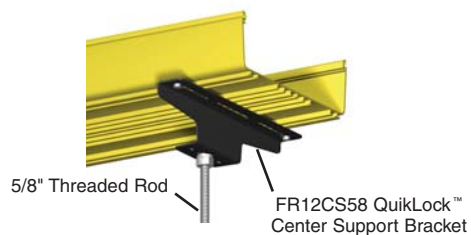
Center Support
