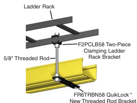
Ladder Rack Support
