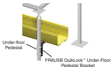
Under-floor Support
