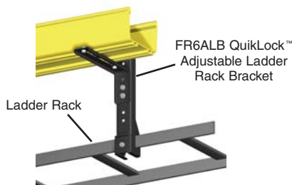
Ladder Rack Support
