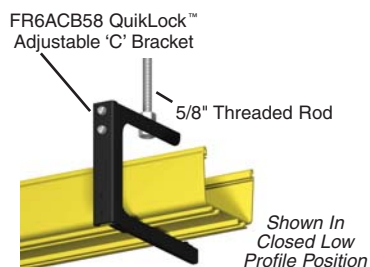
Top Support 'C' Bracket
