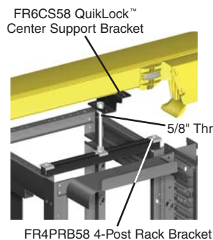
Mounting to Panduit 4 Post Rack
