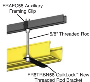
Auxiliary Framing Support
