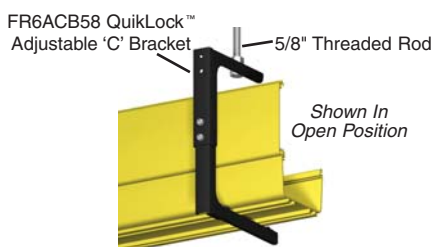
Top Support 'C' Bracket
